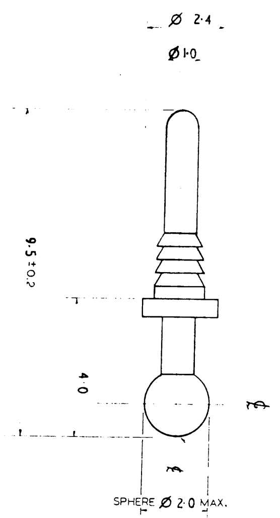
TO SUIT SNAPLOX SOCKET TYPE LS-B-2-156
