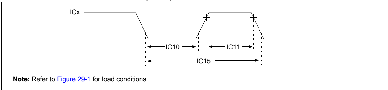
FIGURE 29-7: INPUT CAPTURE (CAPx) TIMING CHARACTERISTICS
