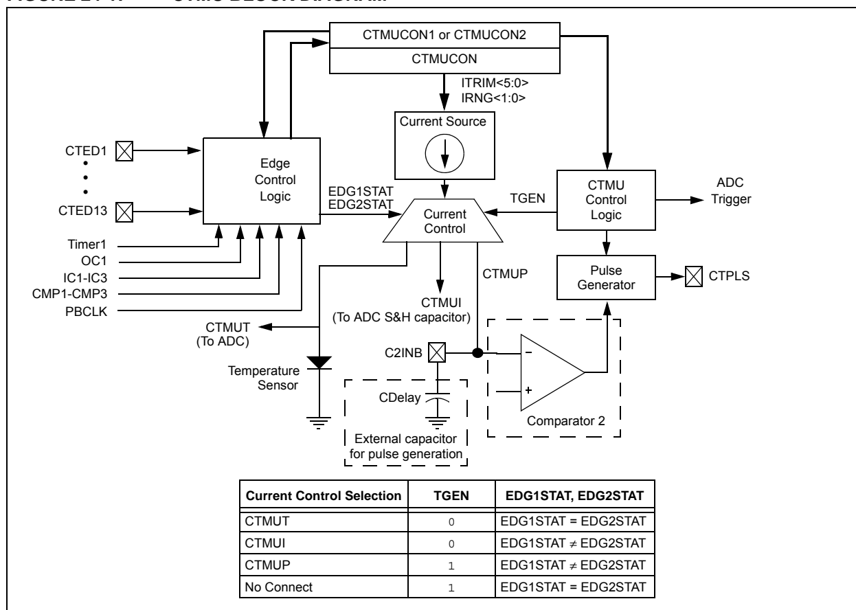
FIGURE 24-1: CTMU BLOCK DIAGRAM
