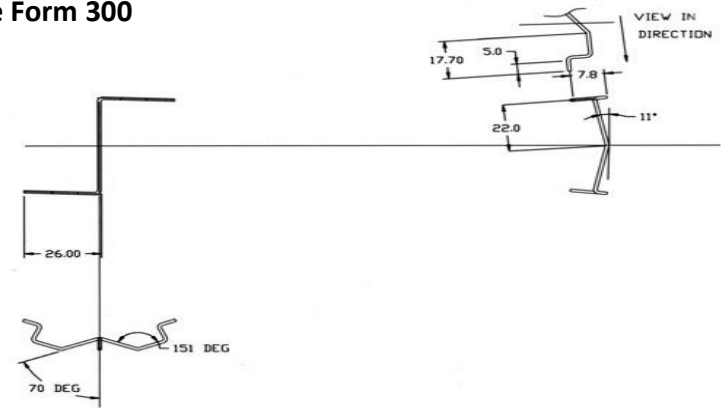
Wire Form 300
