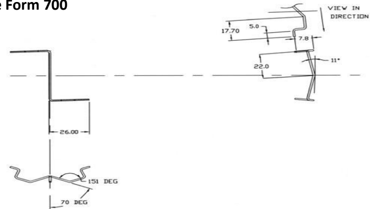
Wire Form 700
