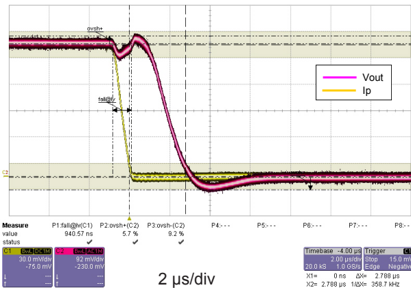
Figure 8: Step response
