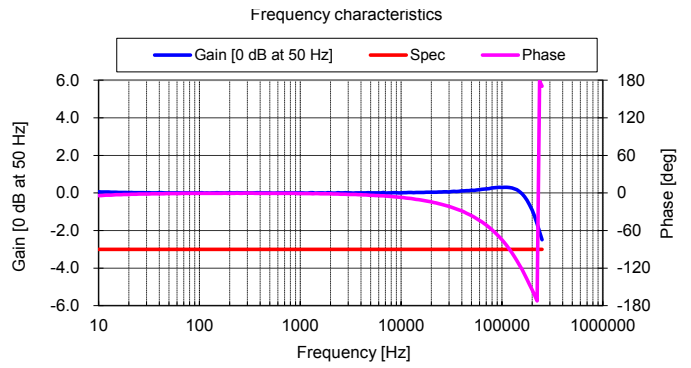
Figure 2: Frequency response
