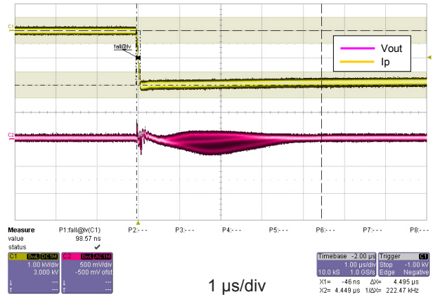
Figure 9: dv/dt
