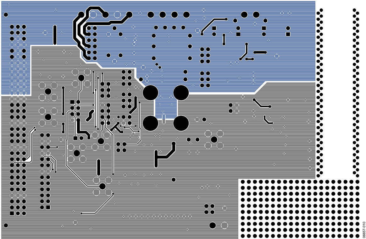
Figure 10. Solder Side
