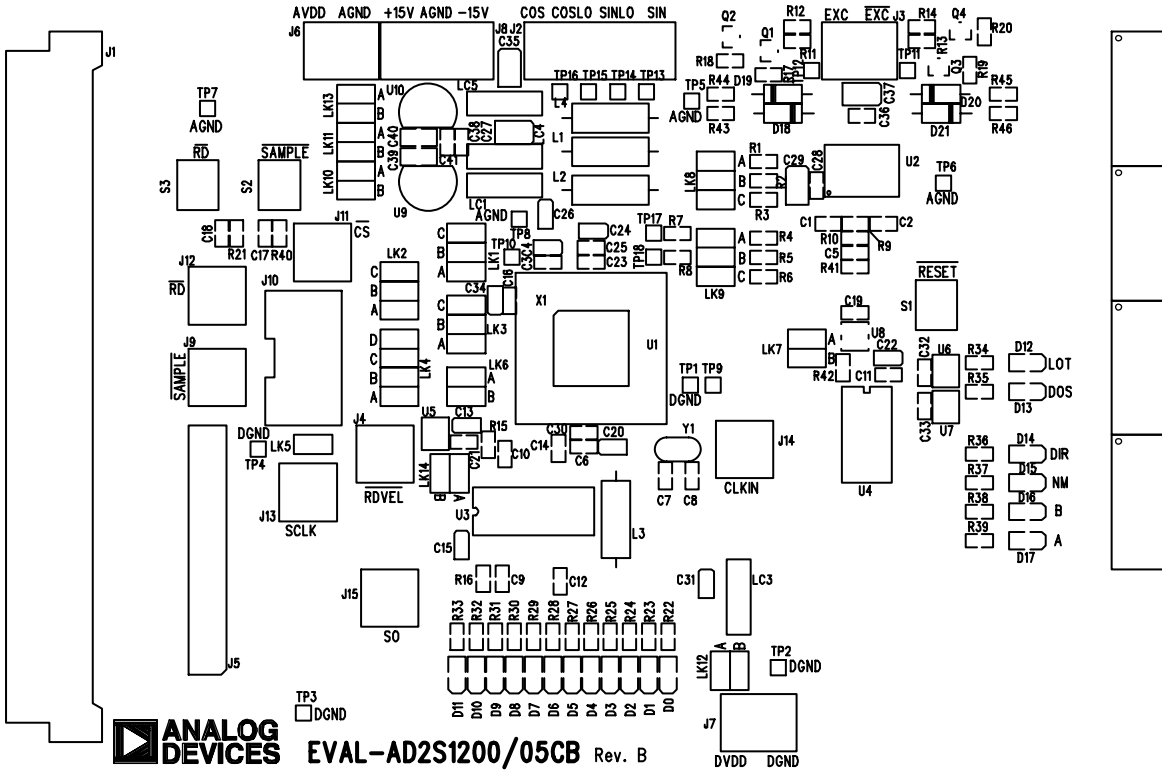
Figure 8. Silkscreen Image
