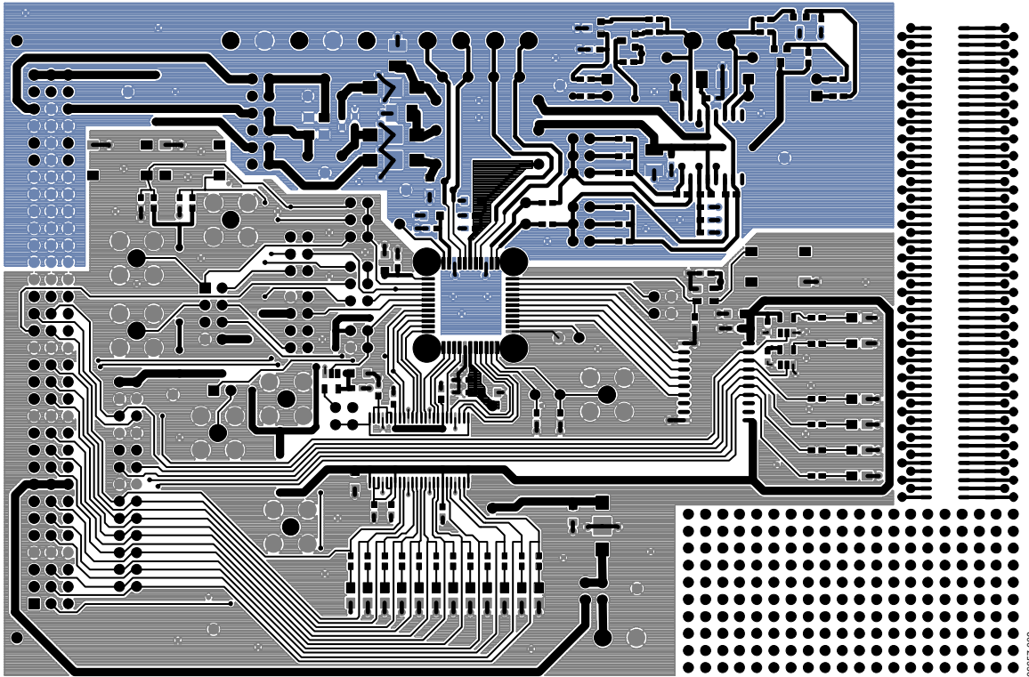
Figure 9. Component Side
