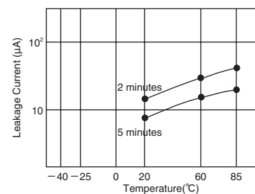
Fig-13 Temperature Characteristics of Leakage Current
