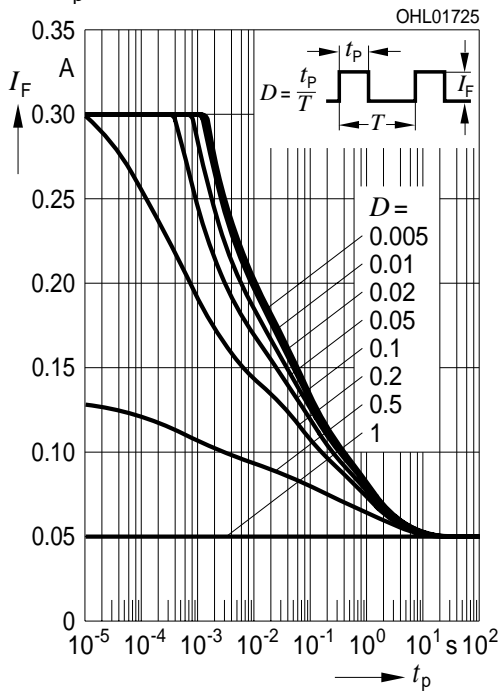
Zulässige Impulsbelastbarkeit Permissible Pulse Handling Capability Duty cycle D = parameter, T_A = 25\text{ °C} I_F = f(t_p) ; true green (3 Chips on)
