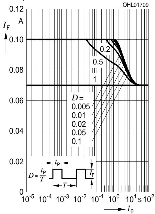
Zulässige Impulsbelastbarkeit Permissible Pulse Handling Capability Duty cycle D = parameter, T_A = 25\text{ °C} I_F = f(t_p) ; red (3 Chips on)
