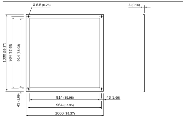
PL880 FS01 Reflector plate, 11 x 11 PL80A, screw connection
