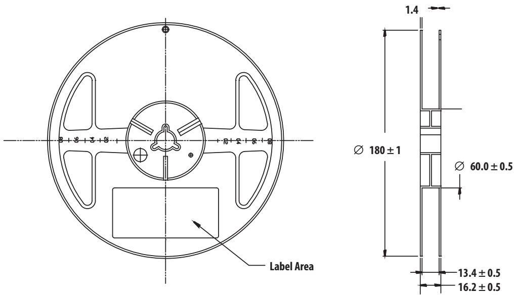
Figure 12. Reel Dimension
