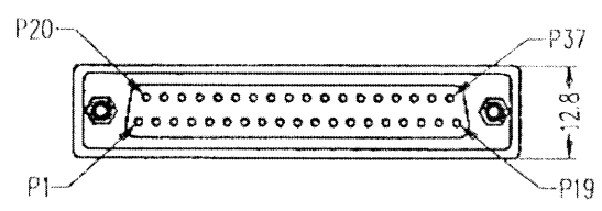
J1-DB37P FEMALE
