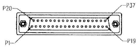
J2-DB37P FEMALE
