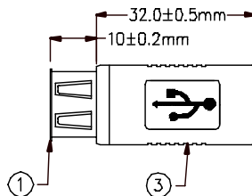
USB A Receptacle
