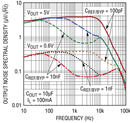
Output Noise Spectral Density vs C_{REF/BYP} = 0, C_{FF} = 0
