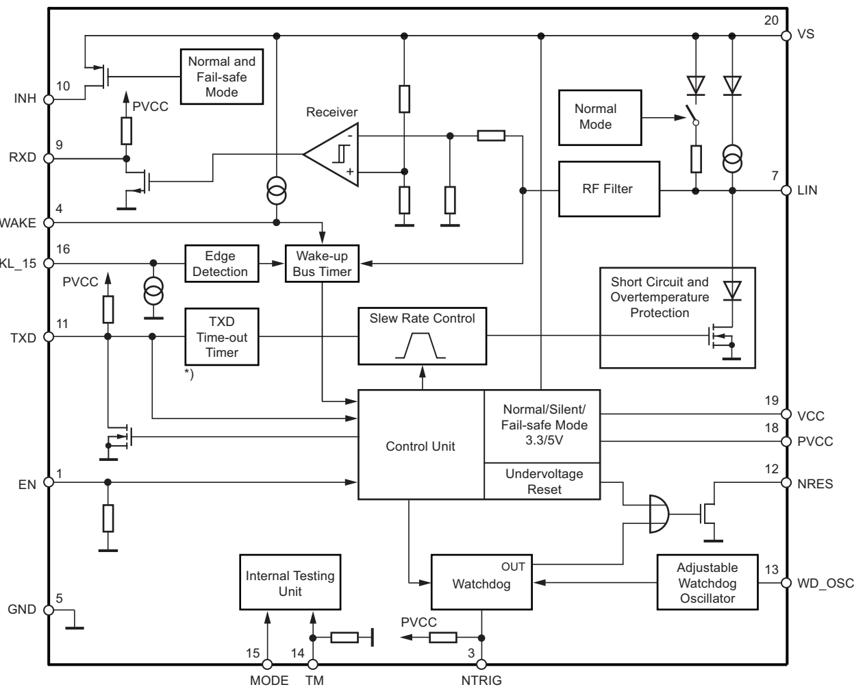
Figure 1-1. Block Diagram
