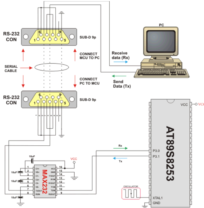
UART HW connection
