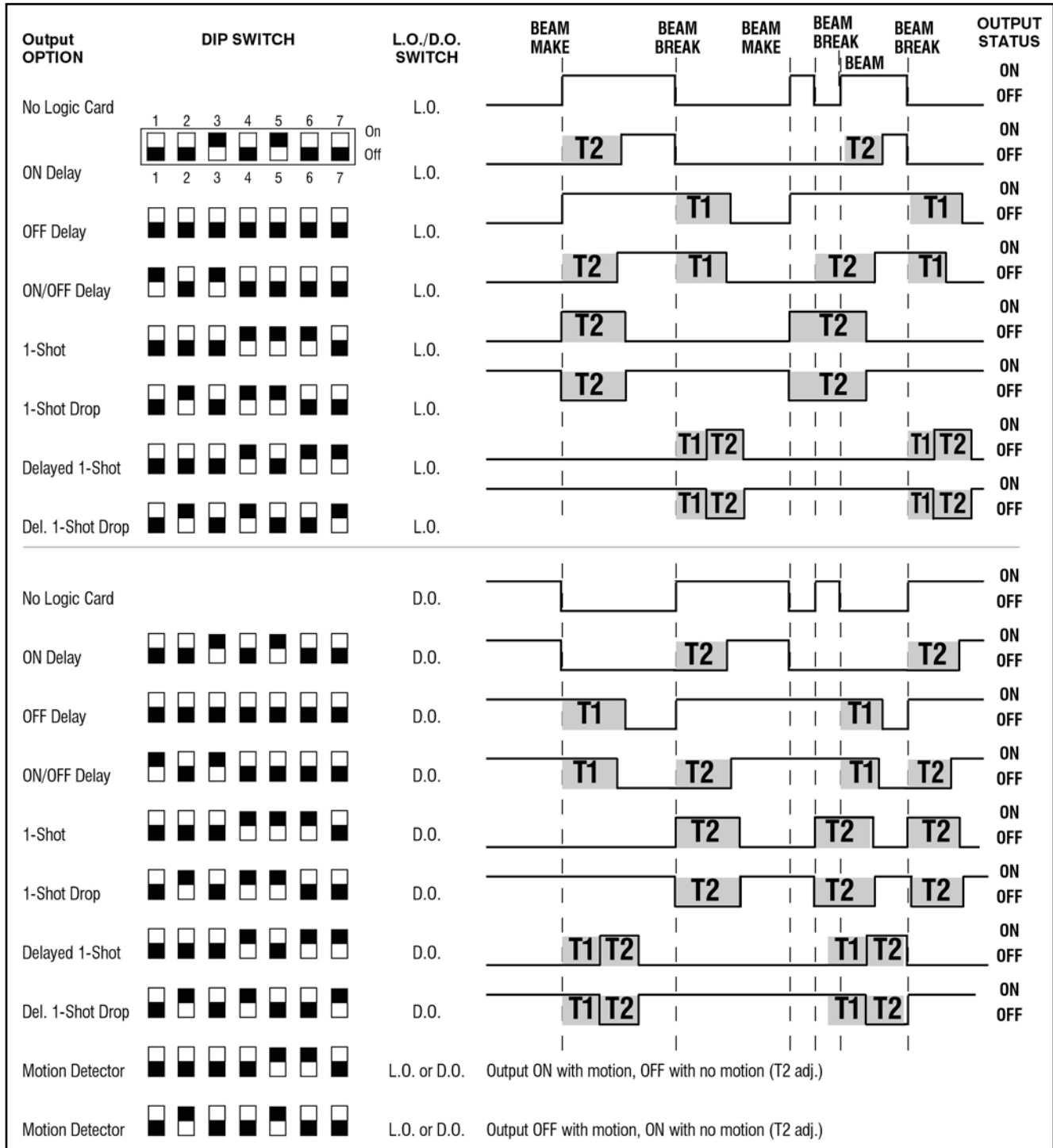
DIP SWITCHES 1-7
