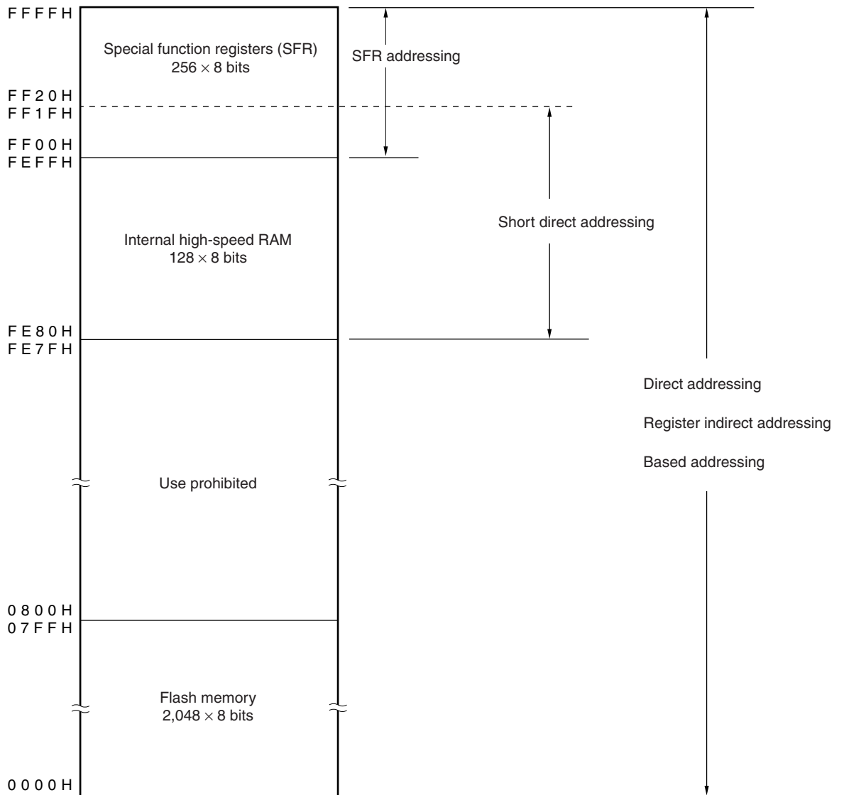
Figure 3-5. Data Memory Addressing ( \mu PD78F9211, 78F9511)
