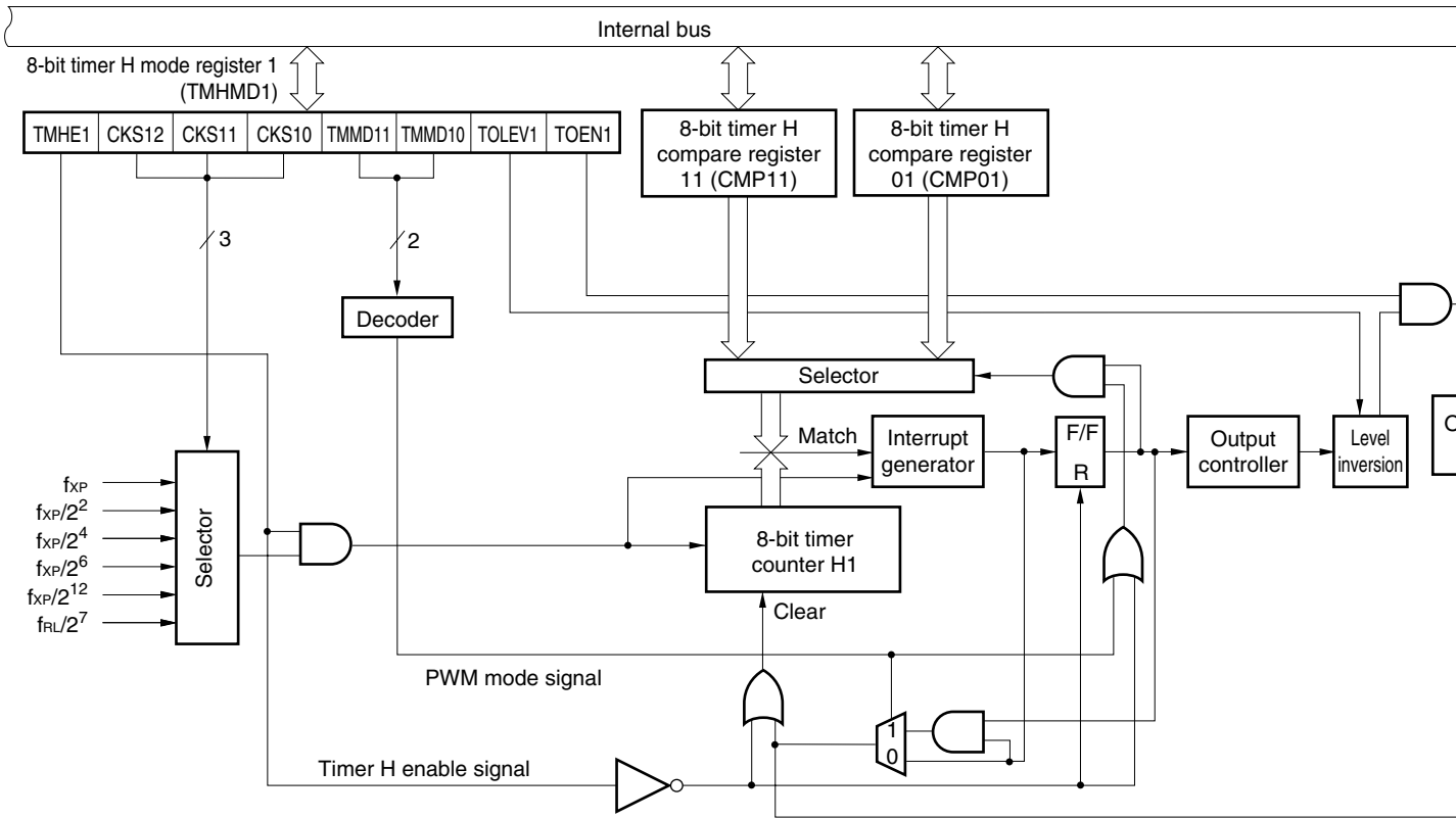
Figure 7-1. Block Diagram of 8-bit Timer H1
