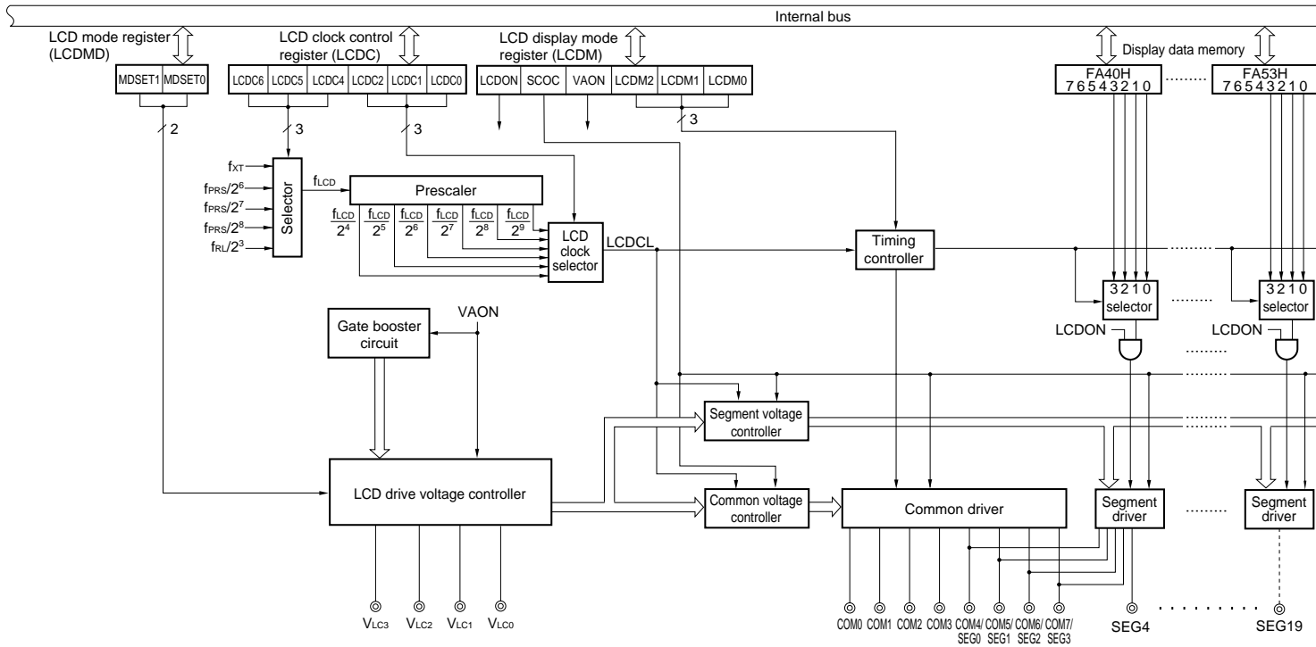
Figure 15-1. Block Diagram of LCD Controller/Driver
