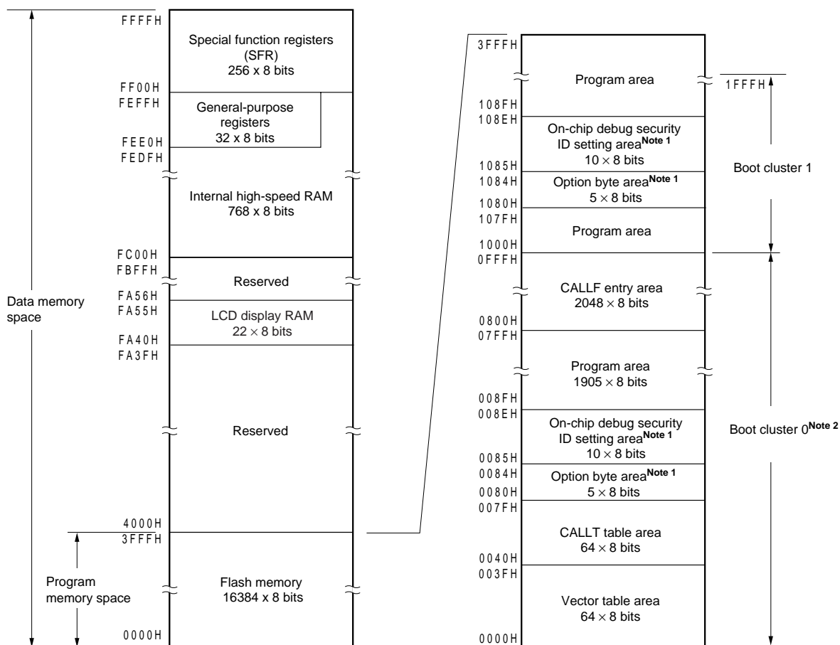
Figure 3-2. Memory Map ( \mu PD78F0401, 78F0411)
