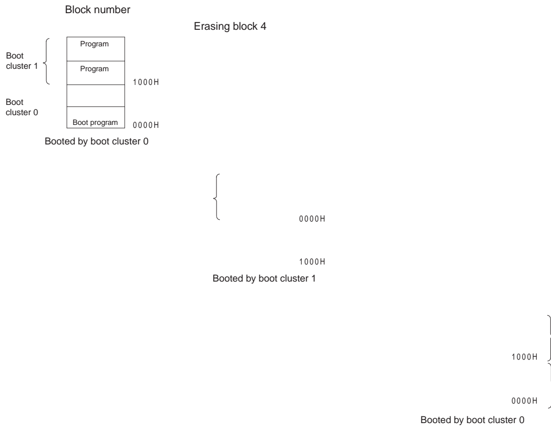
Figure 24-14. Example of Executing Boot Swapping
