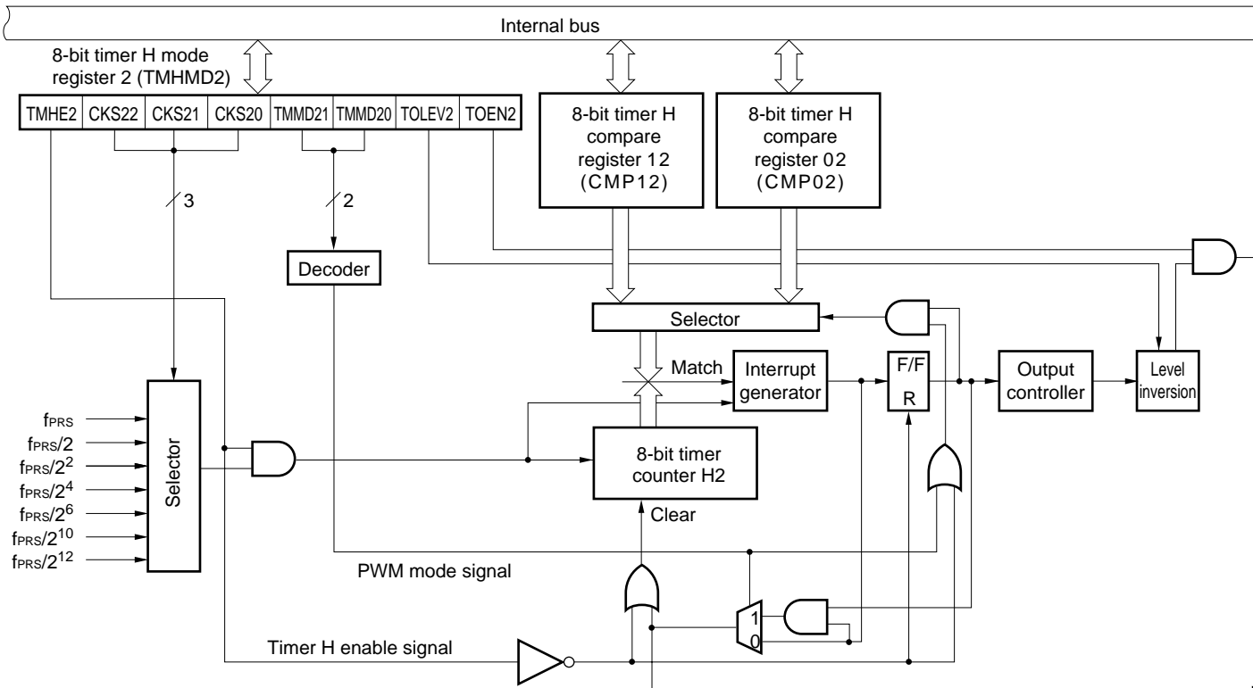
Figure 8-3. Block Diagram of 8-Bit Timer H2
