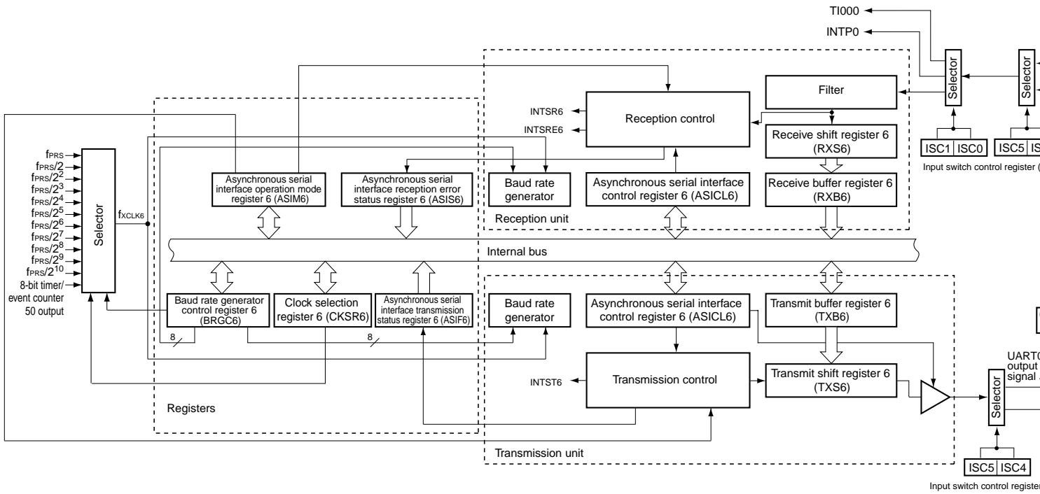
Figure 14-4. Block Diagram of Serial Interface UART6
