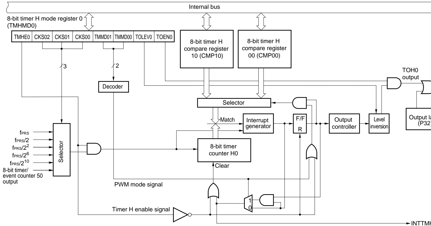
Figure 8-1. Block Diagram of 8-Bit Timer H0
