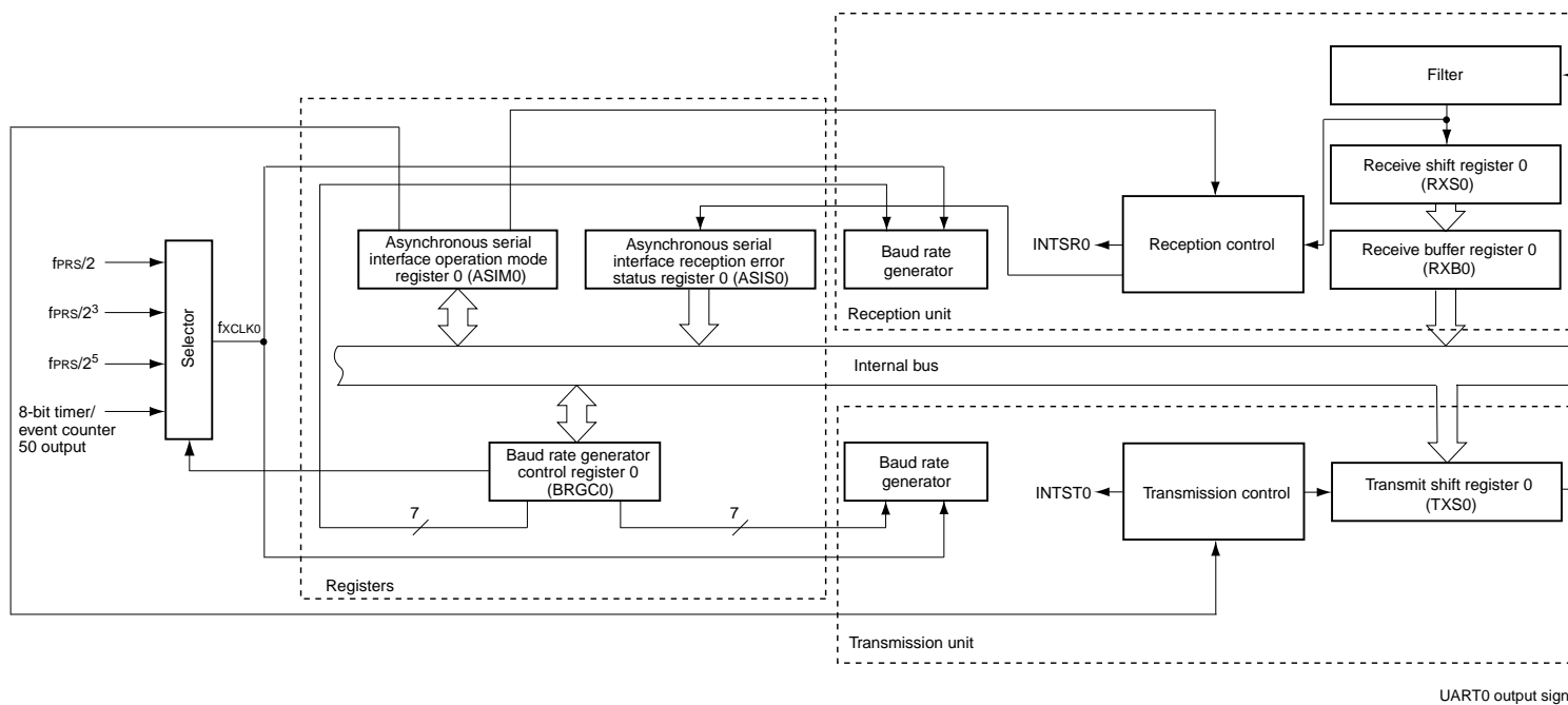
Figure 13-1. Block Diagram of Serial Interface UART0
