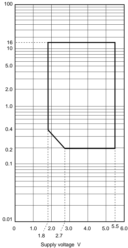
T CY vs. V DD (Main System Clock Operation)
