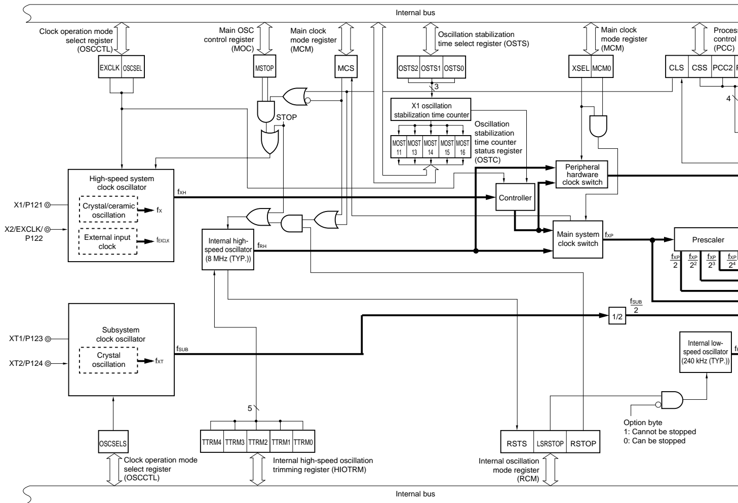
Figure 5-1. Block Diagram of Clock Generator
