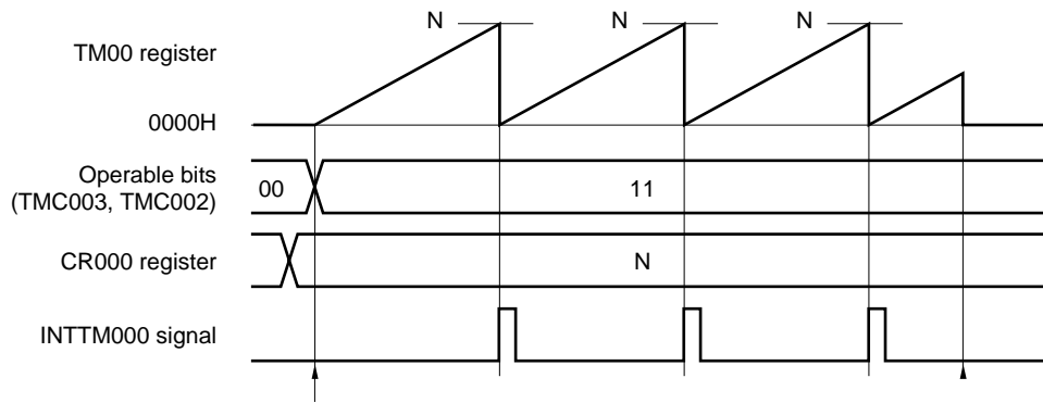
Figure 6-15. Example of Software Processing for Interval Timer Function
