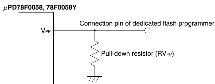
Figure 26-6. V PP Pin Connection Example
