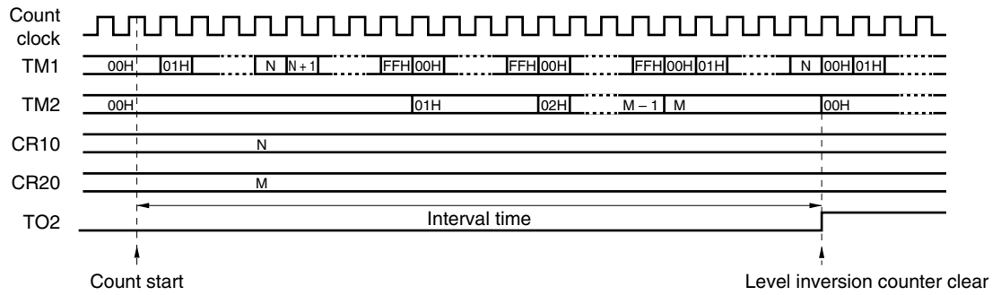
Figure 9-13. Square-Wave Output Operation Timing
