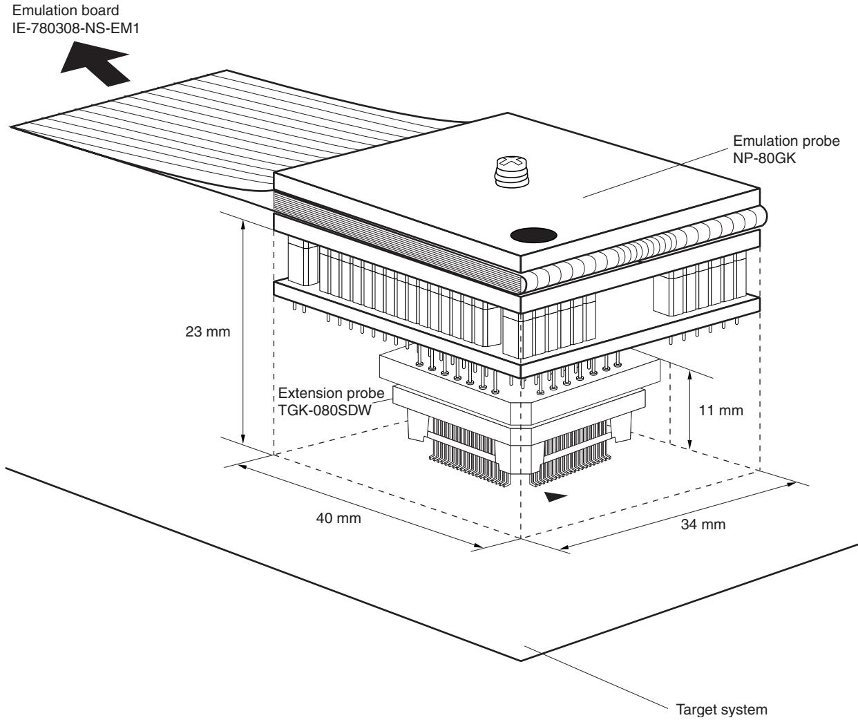
Figure B-9. Connection Condition of Target System (NP-80GK)
