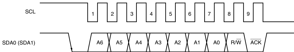
Figure 17-18. Acknowledge Signal
