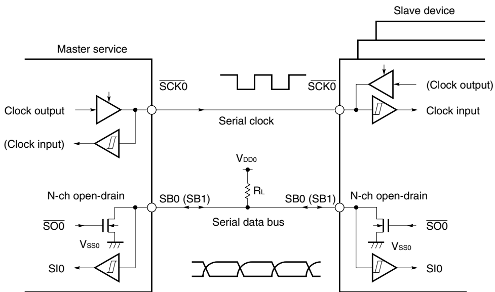
Figure 16-26. Pin Configuration
