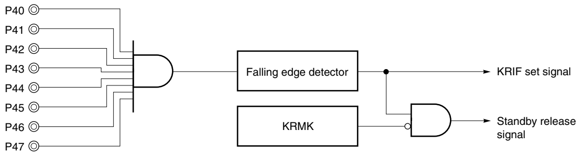
Figure 6-11. Block Diagram of Falling Edge Detector
