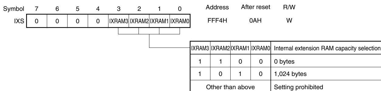
Figure 26-2. Format of Internal Expansion RAM Size Switching Register
