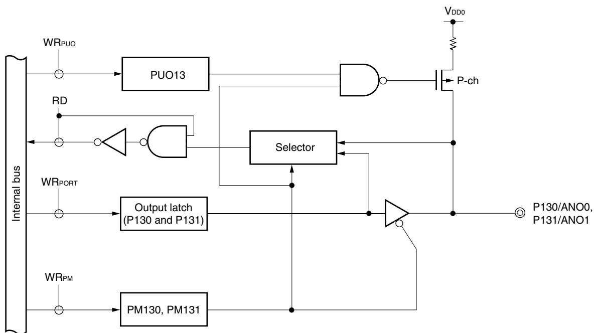
Figure 6-18. Block Diagram of P130 and P131
