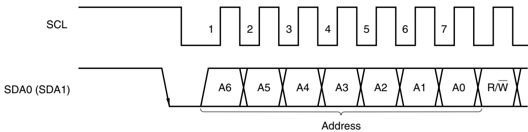
Figure 17-16. Address
