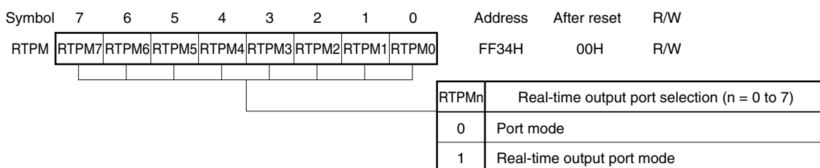
Figure 20-4. Format of Real-Time Output Port Mode Register
