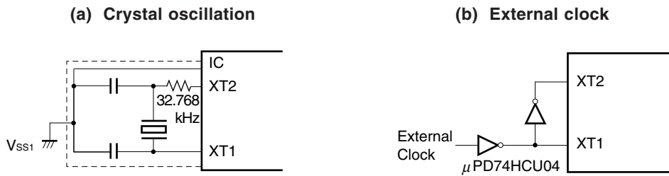
Figure 7-7. External Circuit of Subsystem Clock Oscillator
