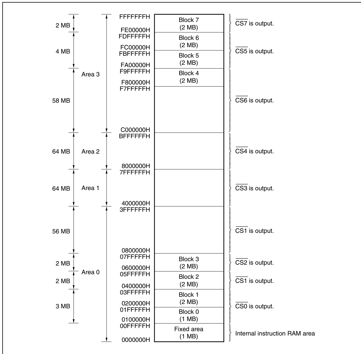
Figure 4-1. Example When CSC0 Register Is Set to 0803H and CSC1 Register Is Set to 0601H
