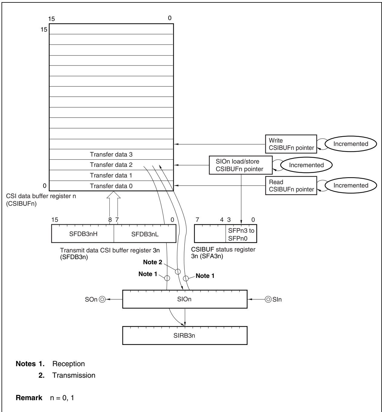
Figure 10-32. Continuous Mode
