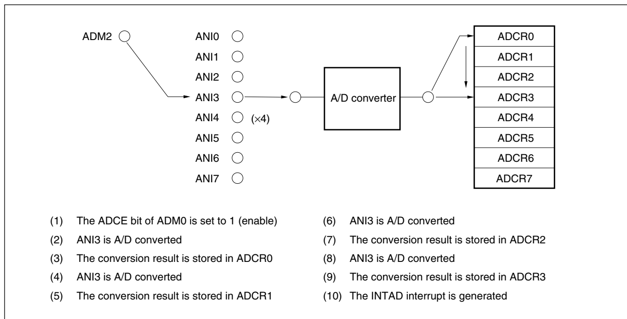
Figure 12-7. Example of 4-Buffer Mode Operation (A/D Trigger Select: 4 Buffers)
