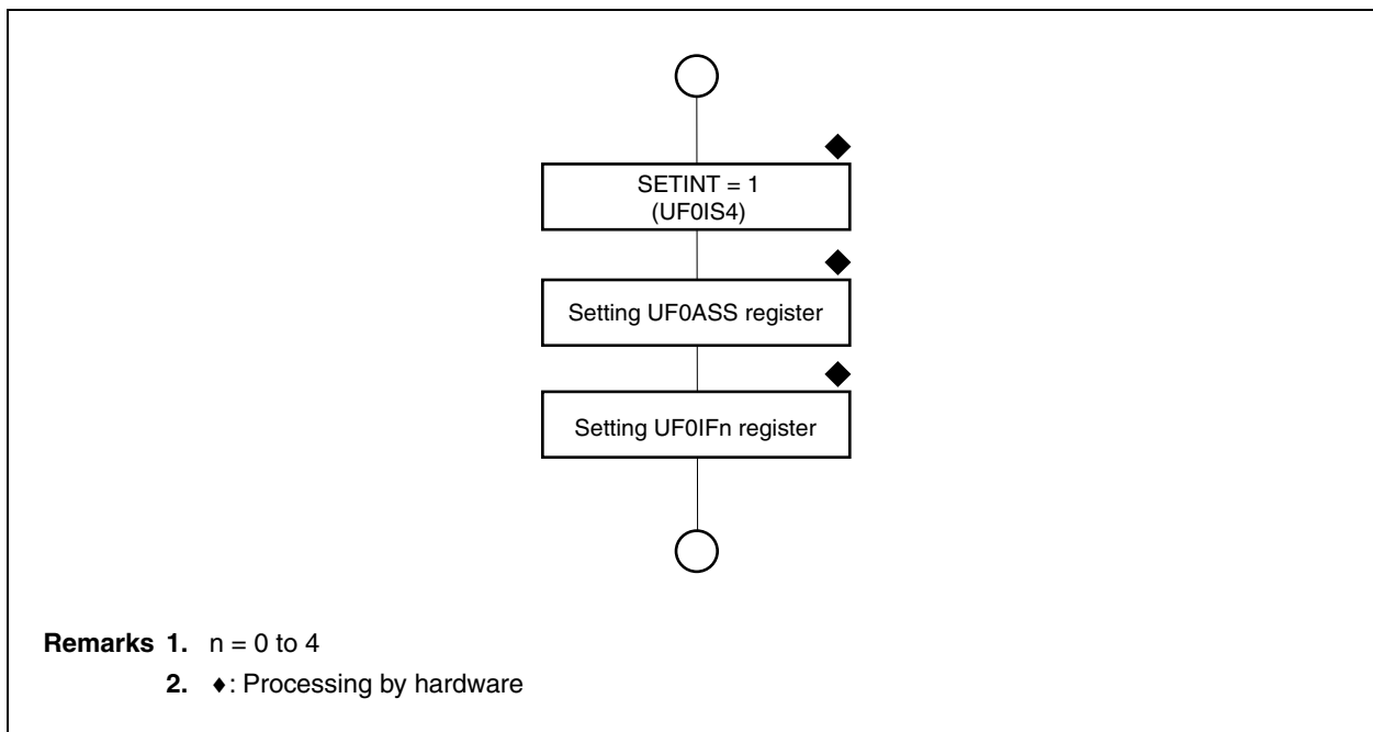
Figure 11-21. SET_INTERFACE Processing
