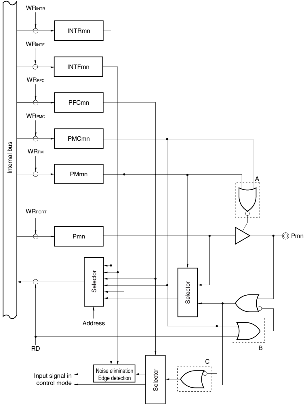
Figure 14-7. Block Diagram of Type F-3
