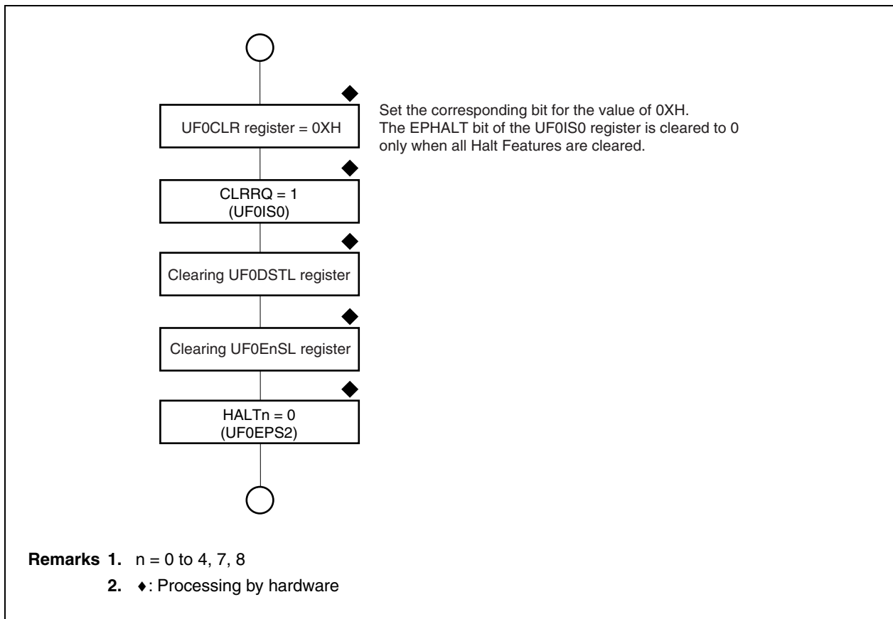
Figure 11-18. CLEAR_FEATURE Processing
