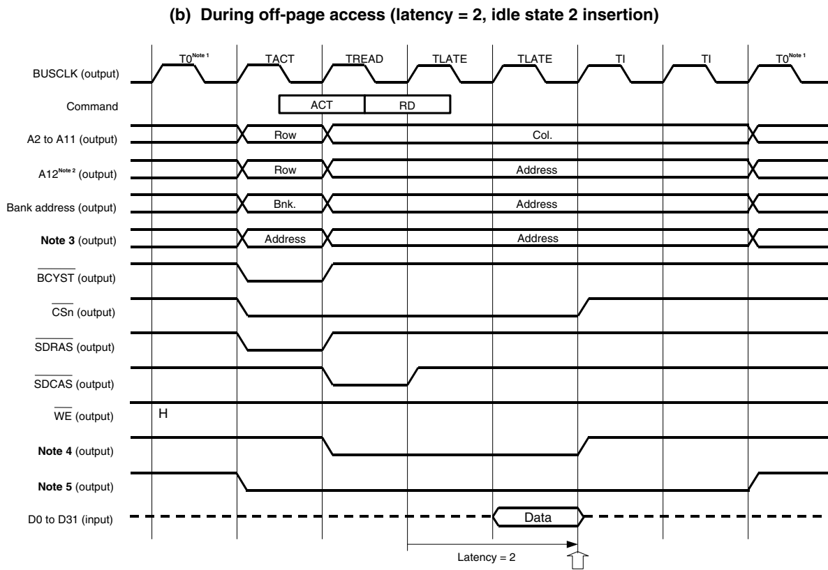
Figure 5-9. SDRAM Single Read Cycle (2/5)
