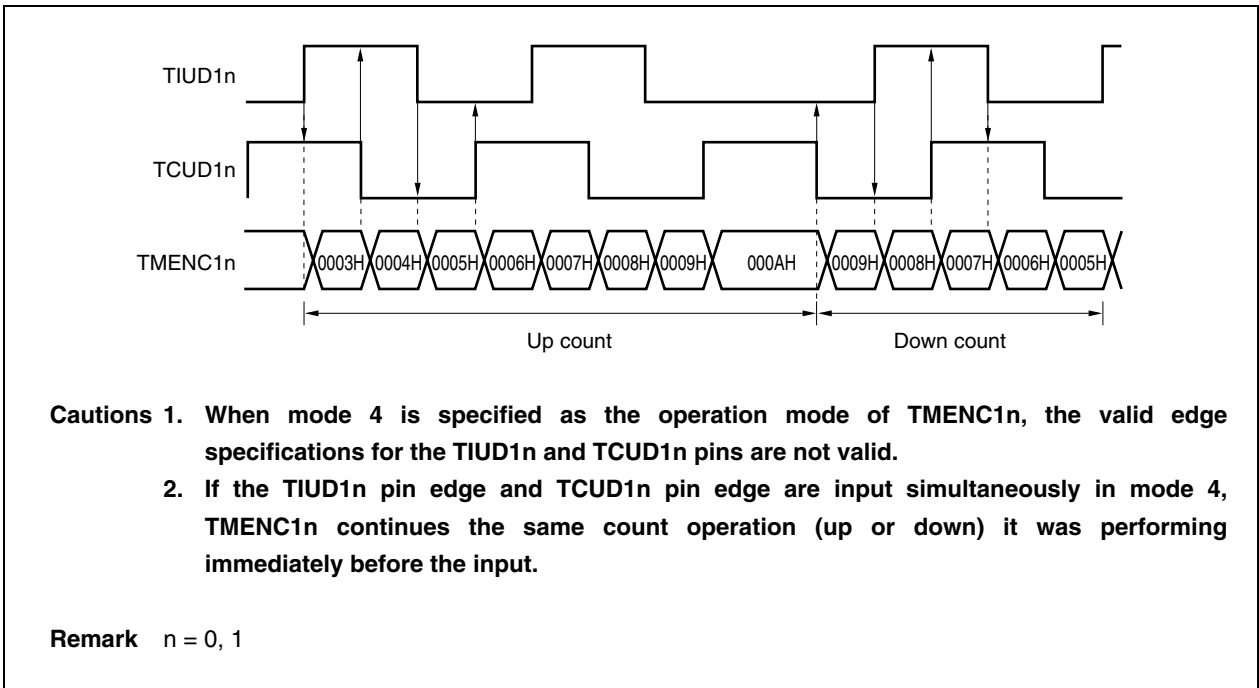
Figure 9-25. Mode 4
