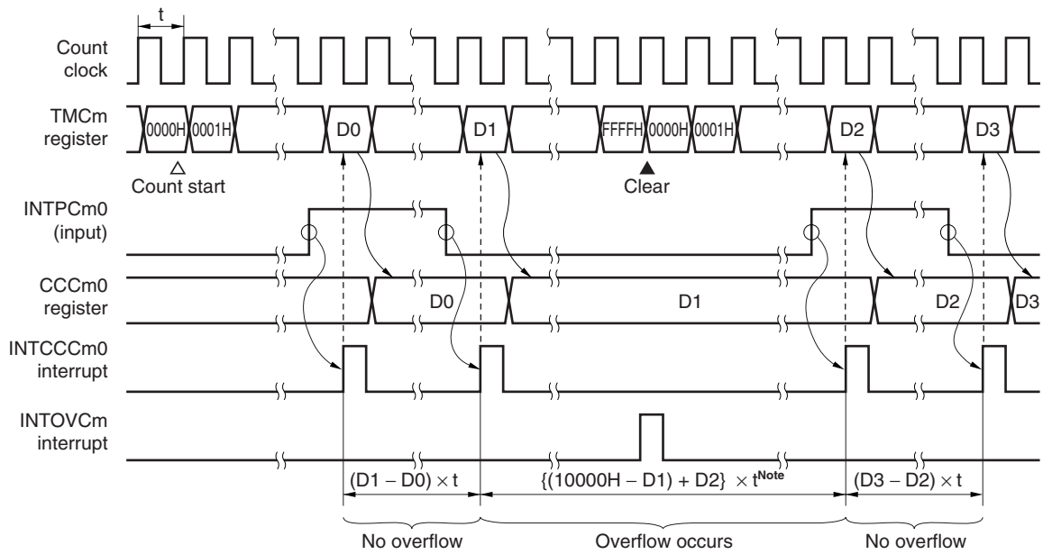
Figure 9-13. Cycle Measurement Operation Timing Example
