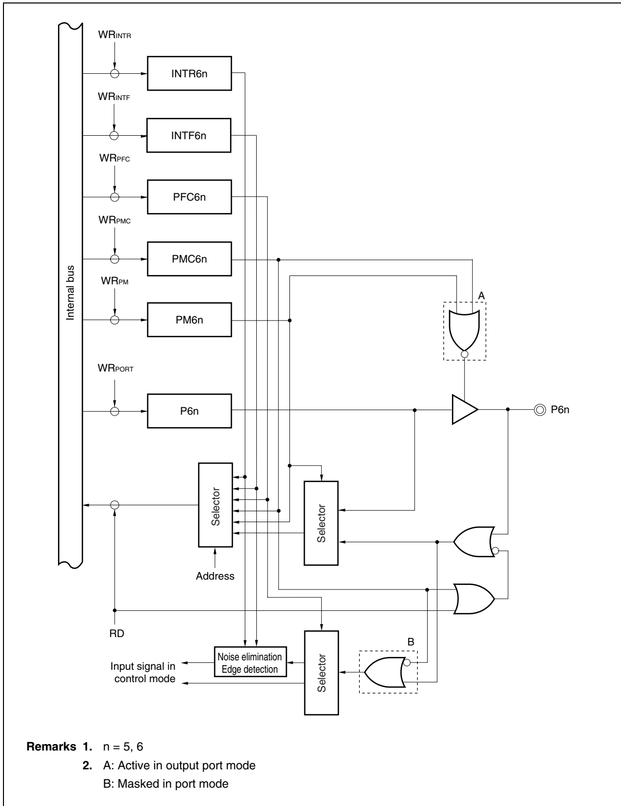
Figure 14-21. Block Diagram of Type L-5
