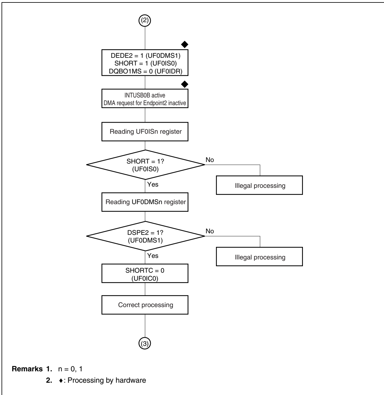
Figure 11-30. DMA Processing by Bulk Transfer (OUT) (2/3)
