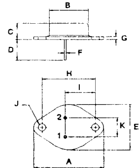
PIN 1.BASE 2.EMITTER COLLECTOR(CASE)
