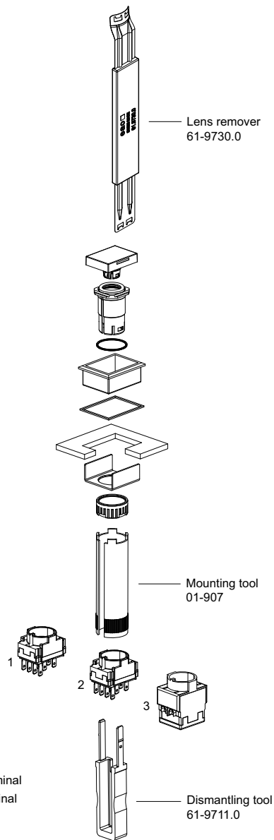
flush mounting
