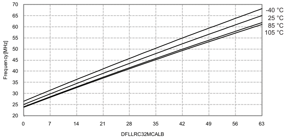
Figure 33-207. 32MHz Internal Oscillator Frequency vs. CALB Calibration Value
