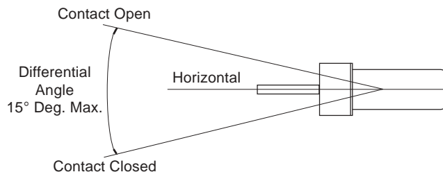
SWITCH OPERATION
