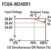
FC6A-M08BR1/FC6A-M24BR1
