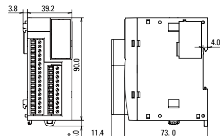
FC6A-M24BR1/FC6A-F2M1 FC6A-F2MR1
