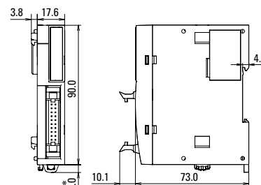
FC6A-N16B3/FC6A-T16K3 FC6A-T16P3
