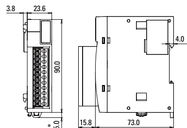
FC6A-N32B3/FC6A-T32K3 FC6A-T32P3
