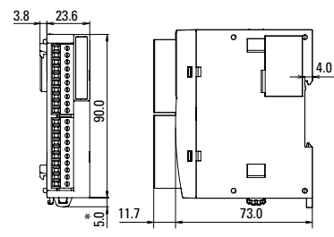
FC6A-M24BR1/FC6A-F2M1 FC6A-F2MR1
