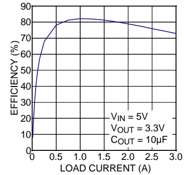
MIC38300 Efficiency
