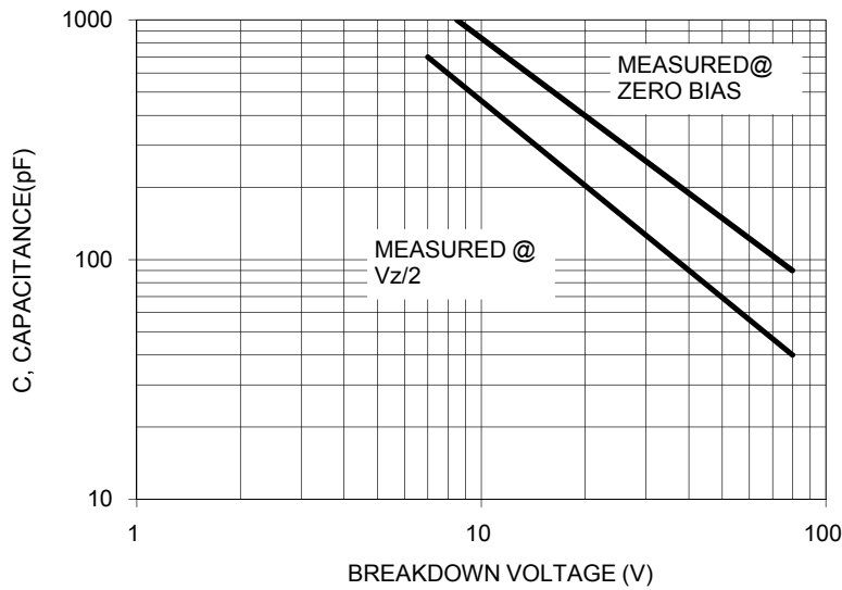
FIG.9 CAPACITANCE CURVE
