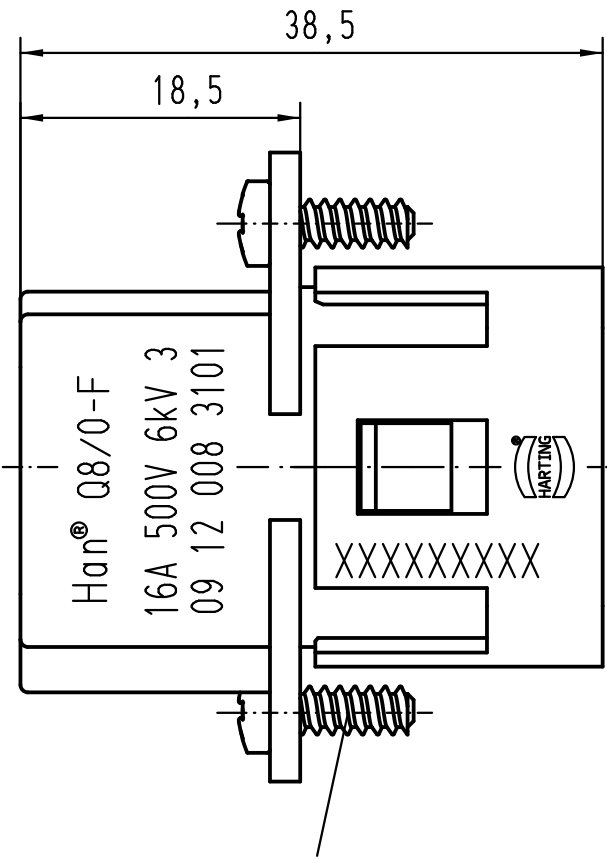
Blechschaube ISO 7049-ST 2,9x9,5-F-H self-tapping screw ISO 7049-ST 2,9x9,5-F-H
