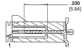
Section K-K
