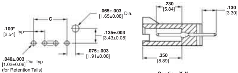
Recommended PC Board Hole Layout
