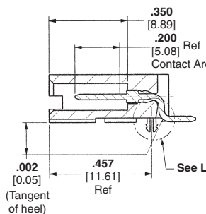
Section K-K
