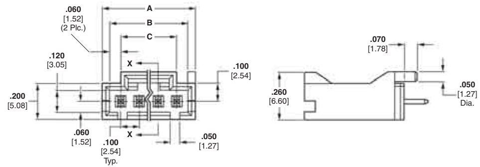
Swaged Retention Tail (See Note)
