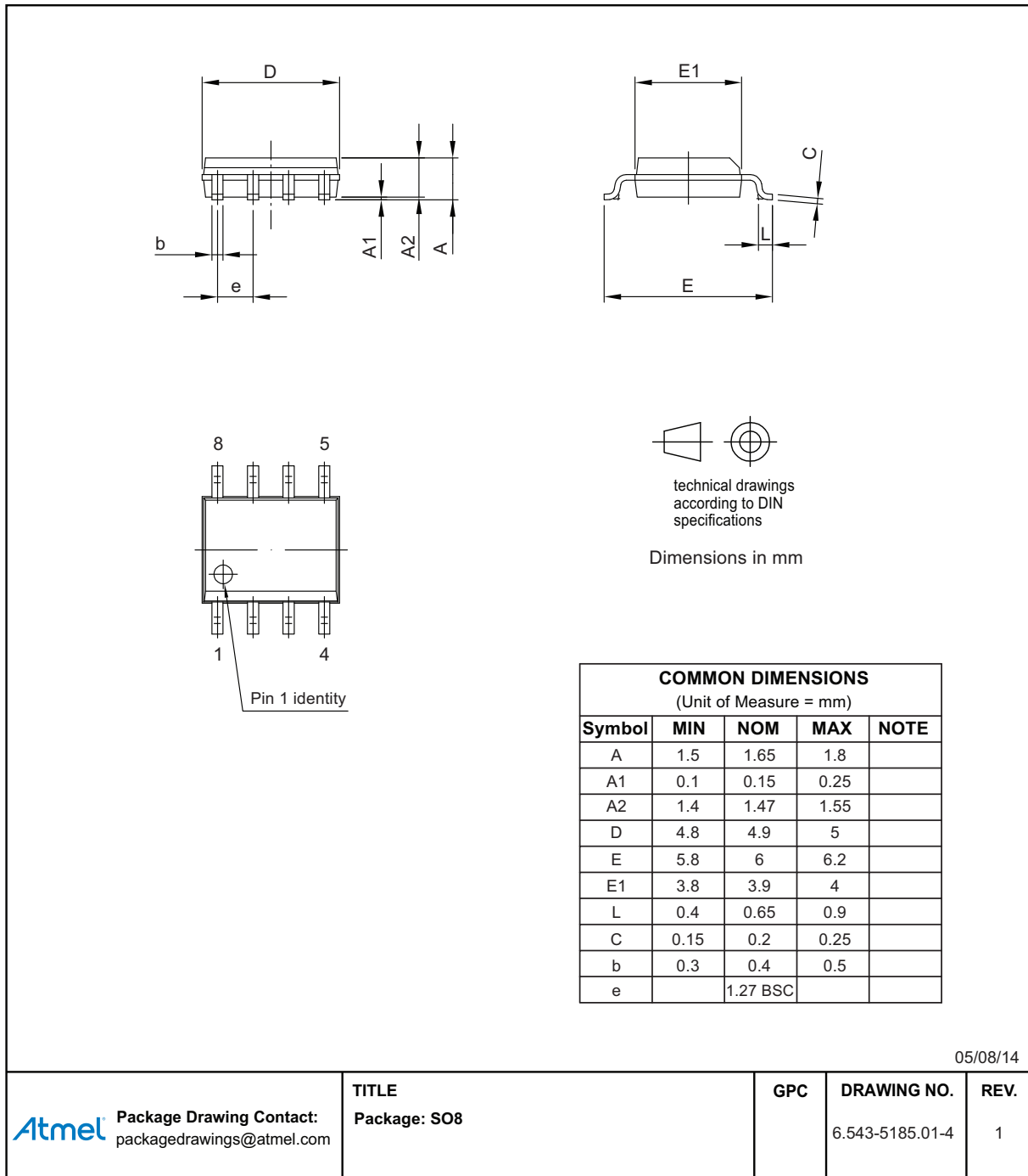
Figure 8-1. SO8
