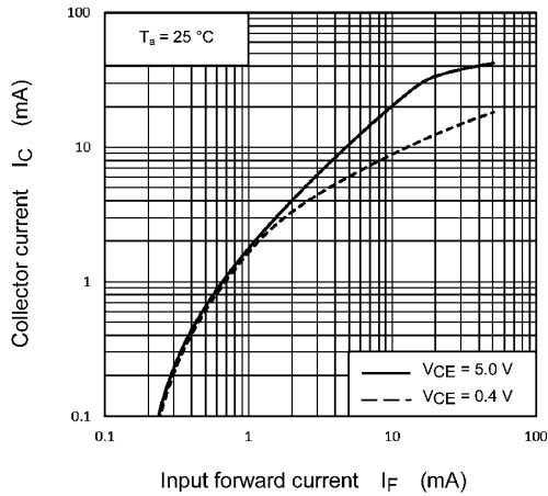
Input forward current I_F (mA) Fig. 11.9 I_C - I_F
