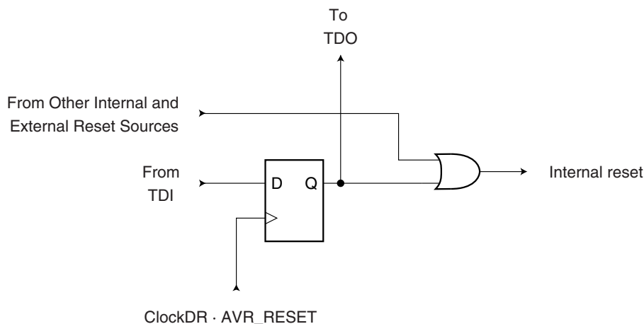
Figure 25-2. Reset register.
