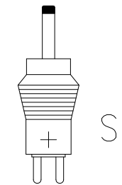
Hohlstecker/ hollowplug Ø1,7xØ4x10mm
