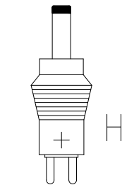
Hohlstecker/ hollowplug Ø2,1xØ5x12mm
