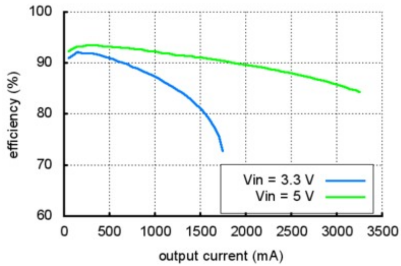
Pololu U3V50F6 Regulator Efficiency (Vout = 6 V)
