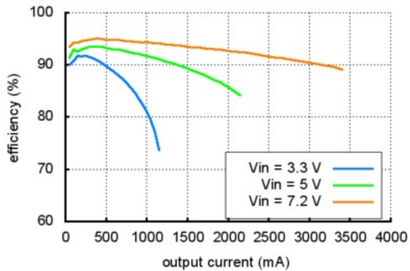
Pololu U3V50F9 Regulator Efficiency (Vout = 9 V)
