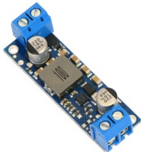
Pololu fixed step-up voltage regulator U3V50Fx, assembled with included terminal blocks.
