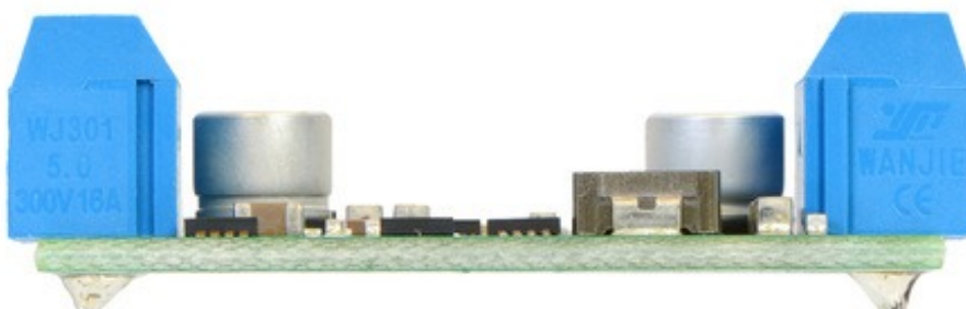
Pololu 5V, 9A Step-Down Voltage Regulator D24V90F5, side view.
