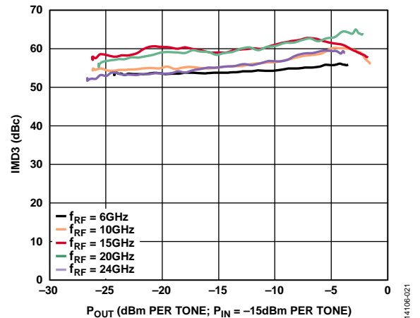
Figure 20. Third-Order Intermodulation Distortion (IMD3) vs. Output Power ( P_{OUT} ) for Various RF Frequencies ( f_{RF} ), BB I/Q Amplitude = -15 dBm per Tone
