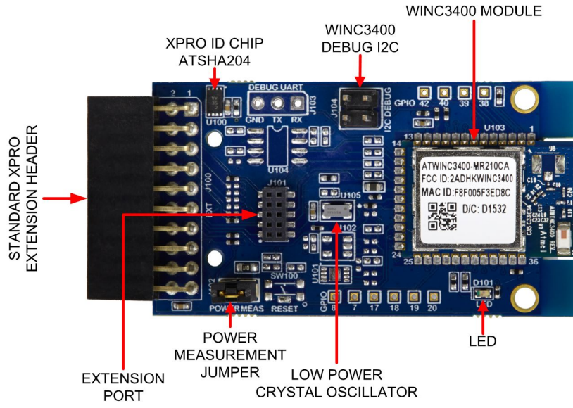
Figure 1-1. ATWINC3400-XPRO
