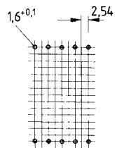
Hole arrangement View in mounting direction
