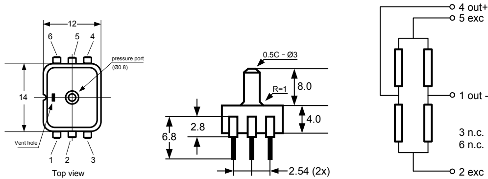
Gauge type sensor
