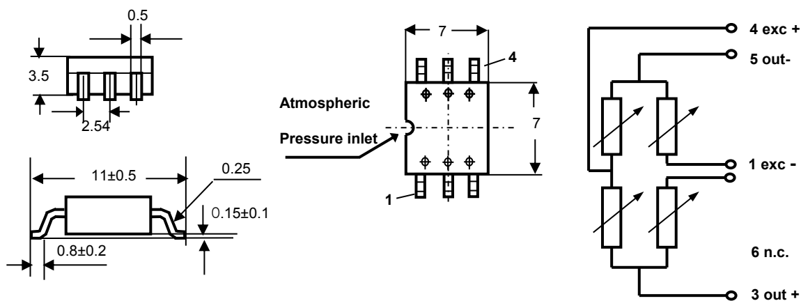
Absolute type sensor (SPD015AB/030AB/100AB)
