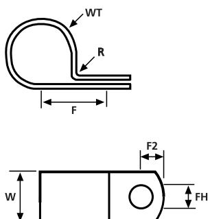
Aluminium P Clips
