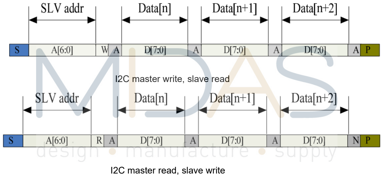
I2C Serial Data Transfer Format
