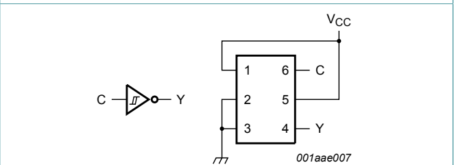
Figure 13. Inverter
