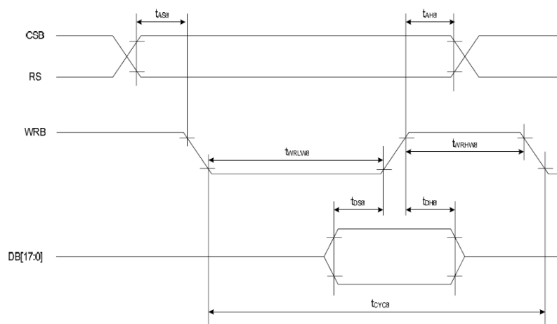
( Write Timing )
