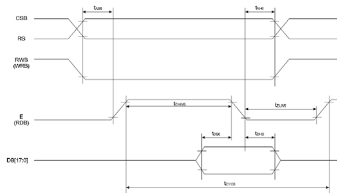
( Write Timing )
