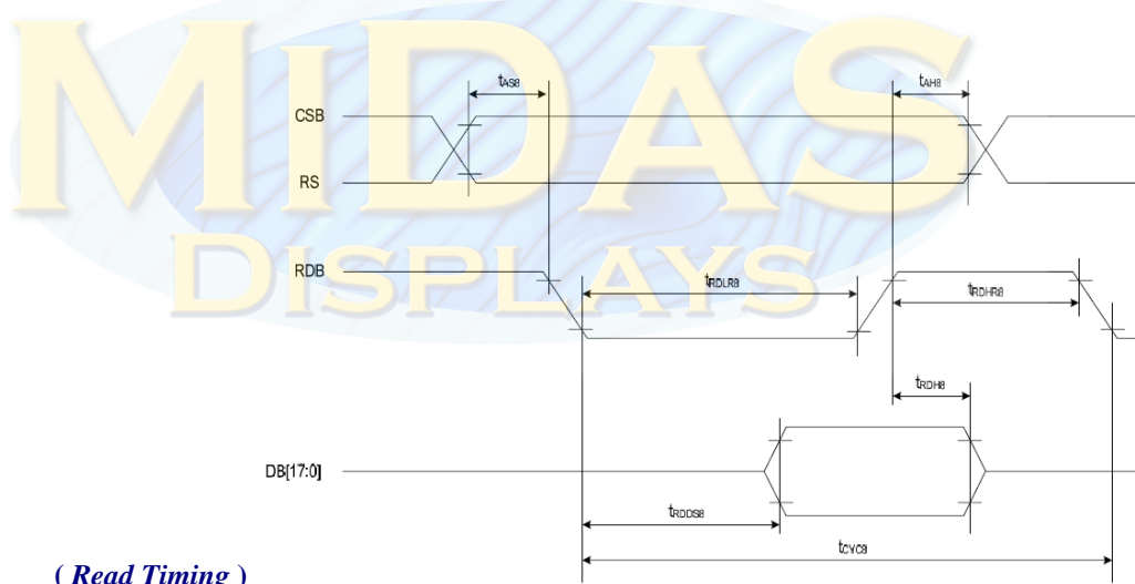
( Read Timing )
