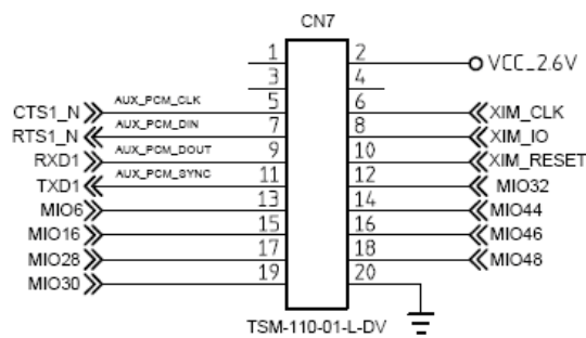
Figure 2-15: Audio test headers
