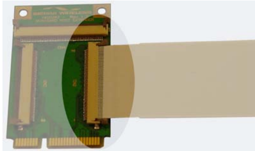
Figure 2-12: Attaching a host extender to a Mini Card
