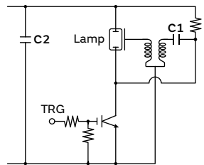
◆Standard current control circuit
