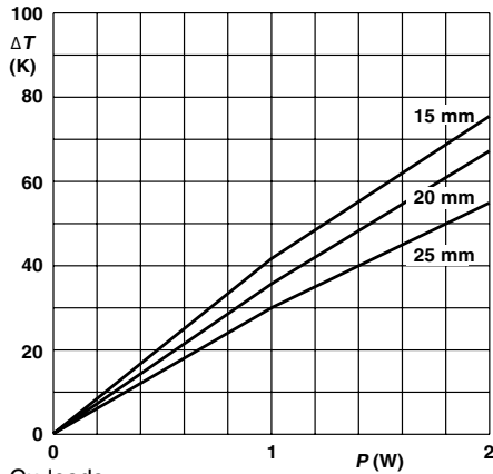
Ø 0.8 mm Cu-leads Minimum distance from resistor body to PCB = 1 mm PR02 Temperature rise ( \Delta T ) at the lead end (soldering point) as a function of dissipated power at various lead lengths after mounting.
