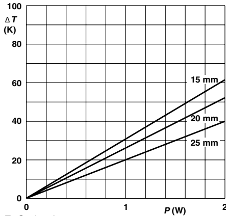
Ø 0.6 mm FeCu-leads Minimum distance from resistor body to PCB = 1 mm PR02 Temperature rise ( \Delta T ) at the lead end (soldering point) as a function of dissipated power at various lead lengths after mounting.
