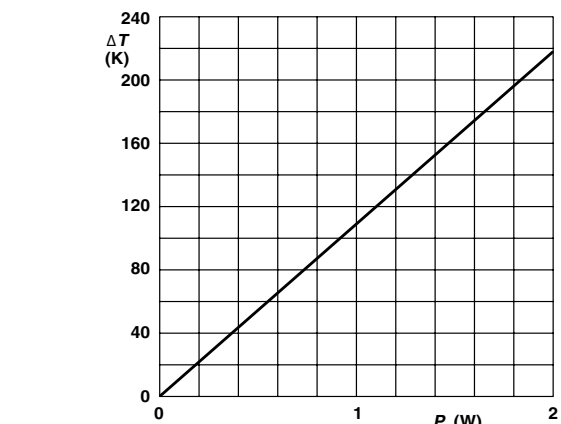
Ø 0.8 mm FeCu-leads PR02 Hot-spot temperature rise ( \Delta T ) as a function of dissipated power.
