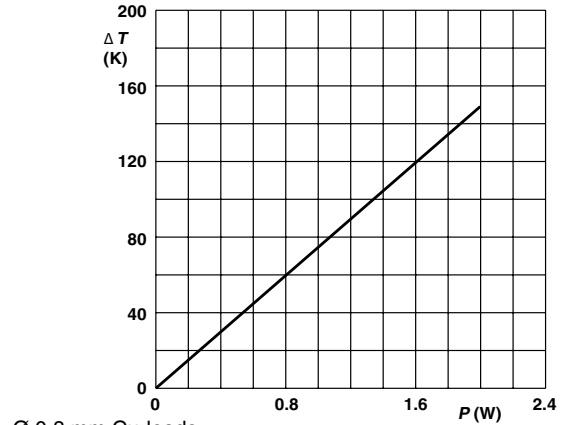
Ø 0.8 mm Cu-leads PR02 Hot-spot temperature rise ( \Delta T ) as a function of dissipated power.
