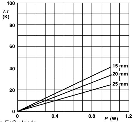
Ø 0.6 mm FeCu-leads Minimum distance from resistor body to PCB = 1 mm PR01 Temperature rise ( \Delta T ) at the lead end (soldering point) as a function of dissipated power at various lead lengths after mounting.
