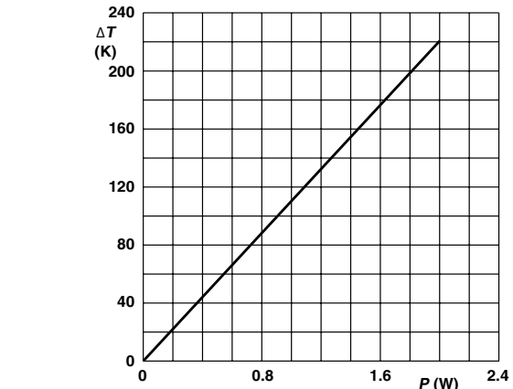
Ø 0.6 mm FeCu-leads PR02 Hot-spot temperature rise ( \Delta T ) as a function of dissipated power.
