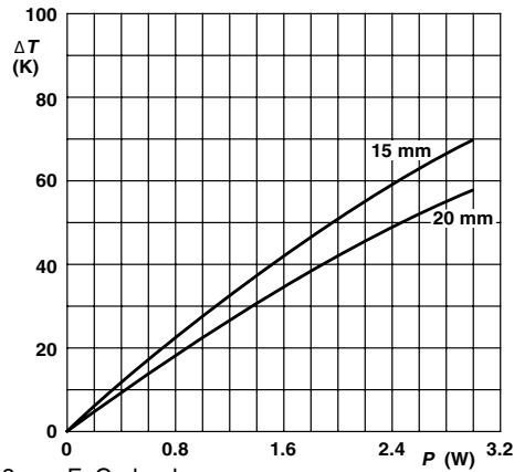
PR03 Temperature rise ( \Delta T ) at the lead end (soldering point) as a function of dissipated power at various lead lengths after mounting.
