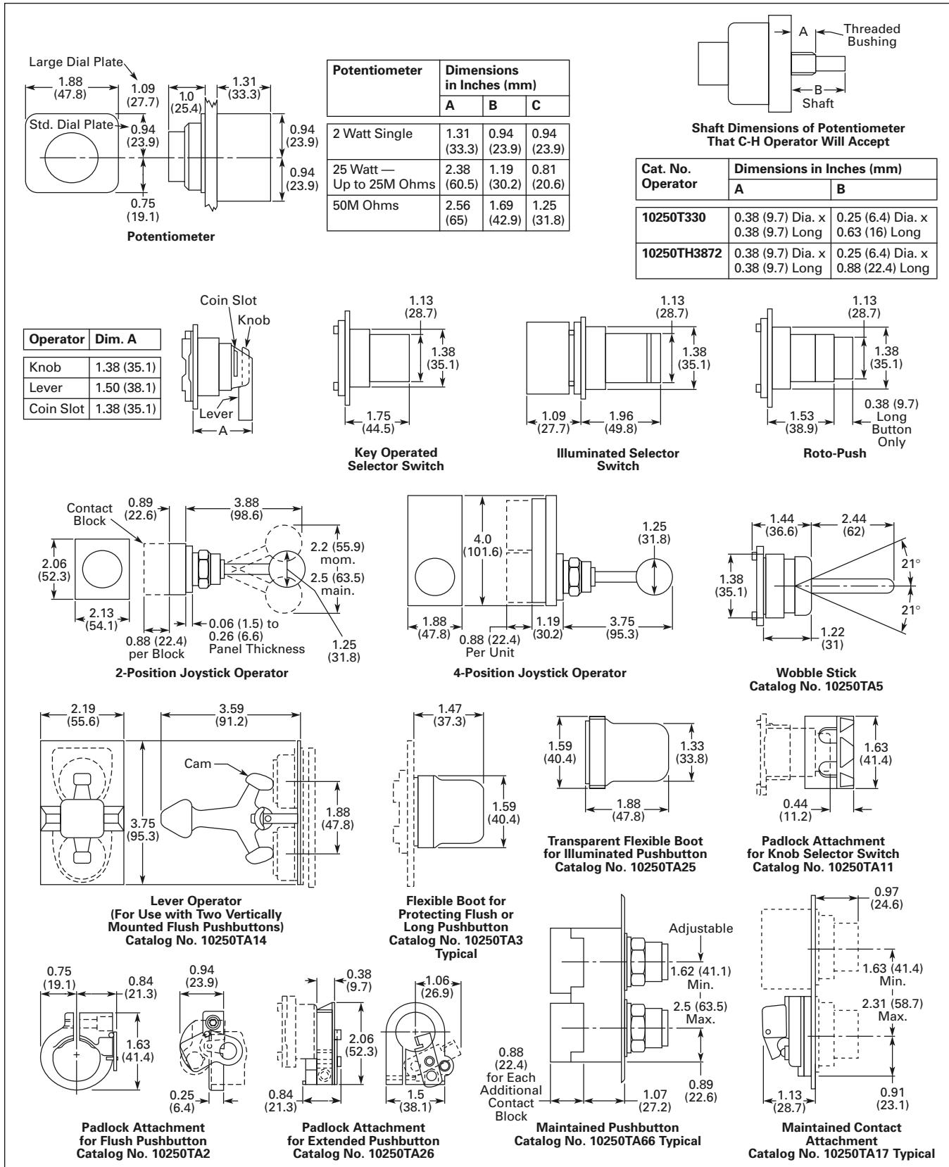
Figure 47-120. Approximate Dimensions in Inches (mm)
