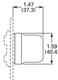
4-Position Joystick Operator
