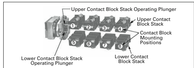
Figure 47-83. Mounting Positions
