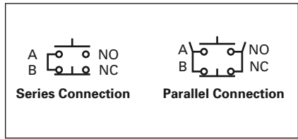
Figure 47-104. Series and Parallel Connections
