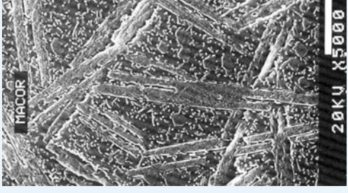
Microstructure of MACOR MGC 5
