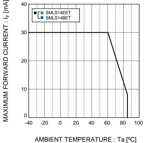
Fig.4 Derating
