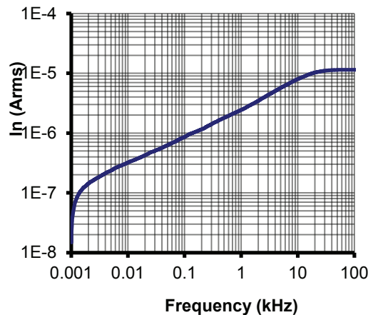
Figure 14: Typical total output current noise (rms) with R_M = 50 \Omega ( f_c is upper cut-off frequency of bandpass, low cut off frequency is 1 Hz)
